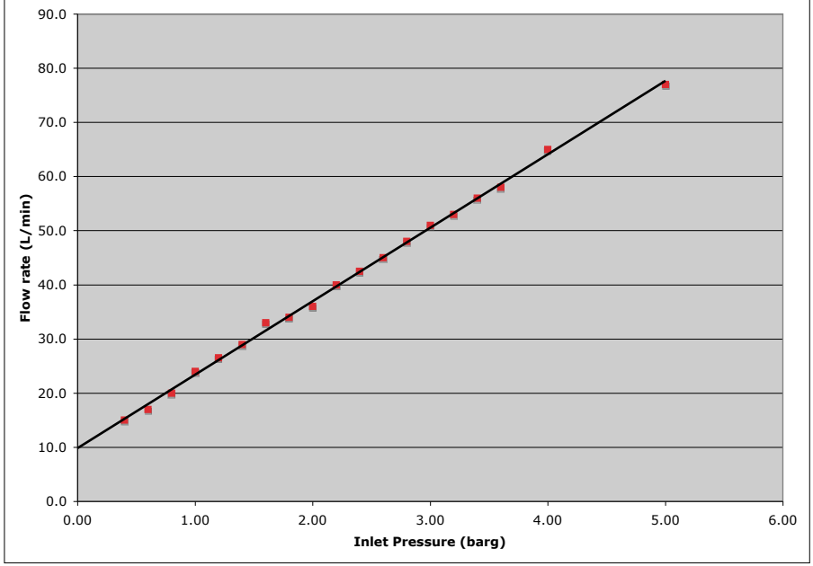
CHECK VALVE PERFORMANCE DATA - 1/4" OD [6.35 mm] AIR FLOW DATA AT 20C, CRACKING PRESSURE = 0.1 BARG
