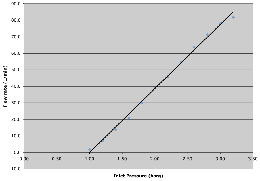
CHECK VALVE PERFORMANCE DATA - 1/4" OD [6.35 mm] AIR FLOW DATA AT 20C, CRACKING PRESSURE = 1 BARG
